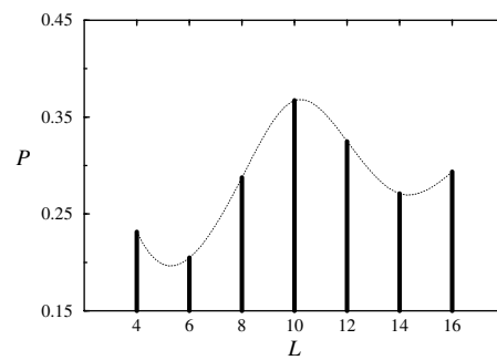
Fig. 4. The dependence of P_5 versus index L of the Daubechies wavelet bases D^L .
