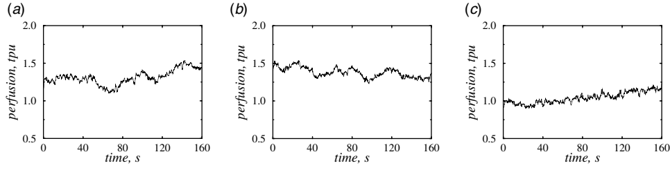
Fig. 1. Examples of LDF-data for a healthy rat (a) and for a rat with UB with (b) and without (c) NO-blockade.
